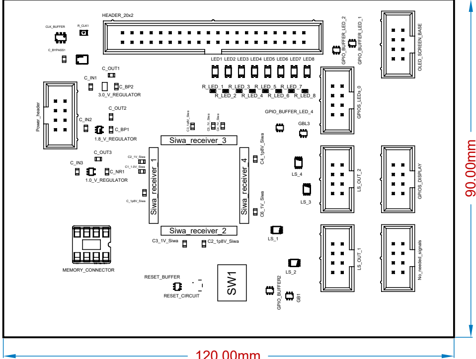
View from Top side (Scale 1:1)
